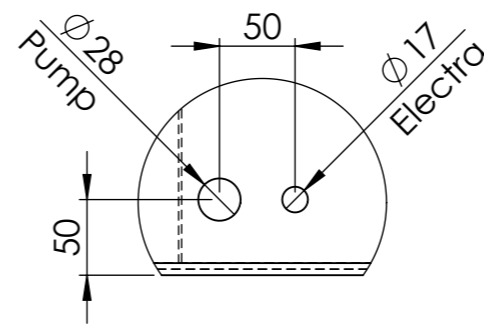
DETAIL C SCALE 1 : 5
